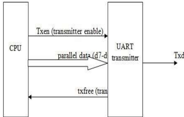
Fig2. UART transmitter
