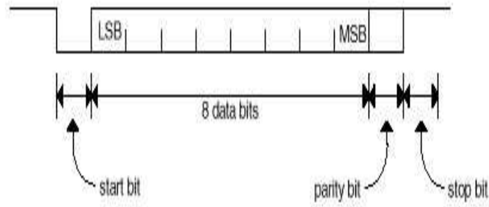
Fig1.Data format of UART
