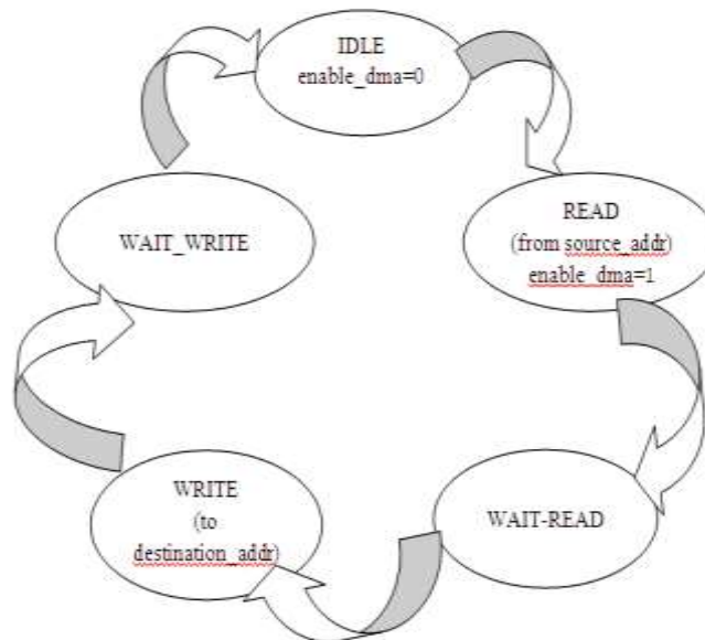
Fig5. State machine of DMA
