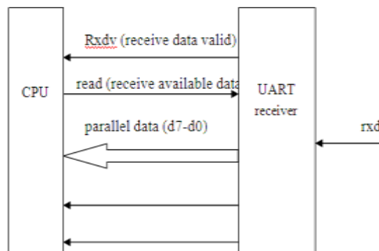
Fig3.UART receiver
